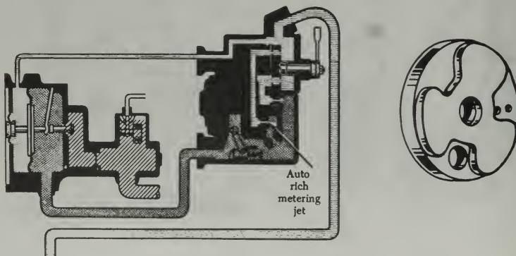
FIGURE 3-27. Manual mixture control, auto-rich setting.
